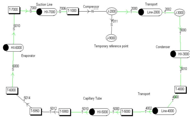
Figure 6. Schematic Diagram of SINDA/FLUENT Transient Air Conditioning System Model
