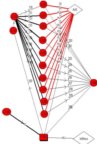
Figure 7. Schematic Diagram of the SINDA/FLUENT Cabin Thermal-Hydraulic Model
